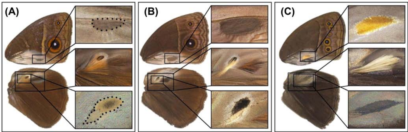
Figure 1. Representation of morphological differences in androconial structures among the investigated species of mycalesine butterflies; (A) Bicyclus anynana , (B) Bicyclus safitza , and (C) Mycalesis perseoides . Androconia are formed of differentiated scales and in mycalesine males they generally consist of linked patches and hair pencils found on both fore- and hindwings. The androconia are involved in the production and release of male sex pheromones (MSP). Left side of each species panel shows the ventral forewing (mirrored) and dorsal hindwing, and the three smaller images to the right show the androconia in detailed view. The upper of the detailed images shows the main androconia on the ventral forewing, the middle shows the dorsal hairpencil(s) on the hindwing, and the lower shows the patch located below the inner hairpencil (hairs removed to aid visibility). The size of the androconial patches was measured as the area within a polygon formed by a series of landmarks (examples shown with black dots in A).
